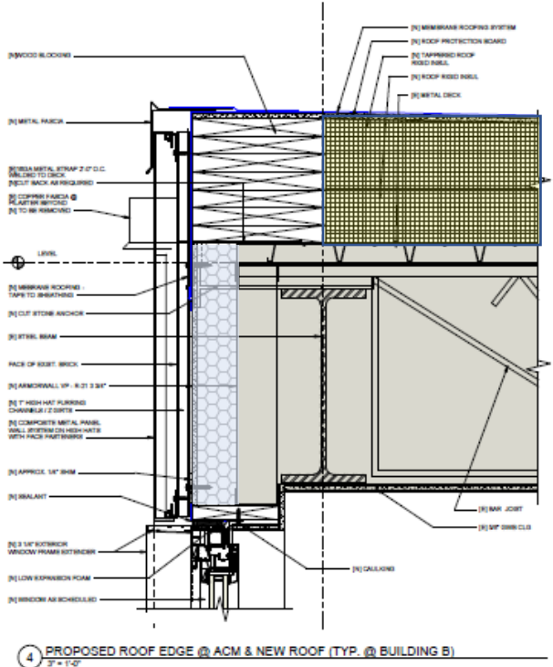
New Roof with Insulation Roof to Wall Detail
